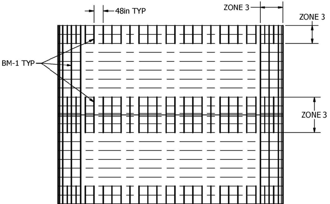
(STEP 1) BM-1 TYPICAL LAYOUT
